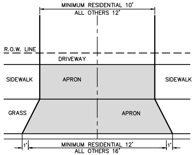
DEPRESSED ENTRANCE LAYOUT NOT TO SCALE
