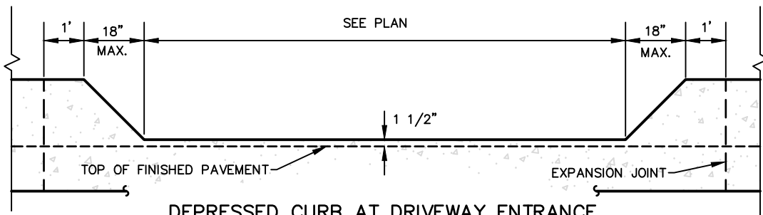
DEPRESSED CURB AT DRIVEWAY ENTRANCE NOT TO SCALE
