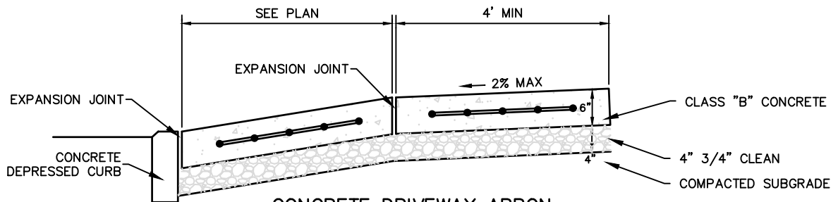
CONCRETE DRIVEWAY APRON NOT TO SCALE
