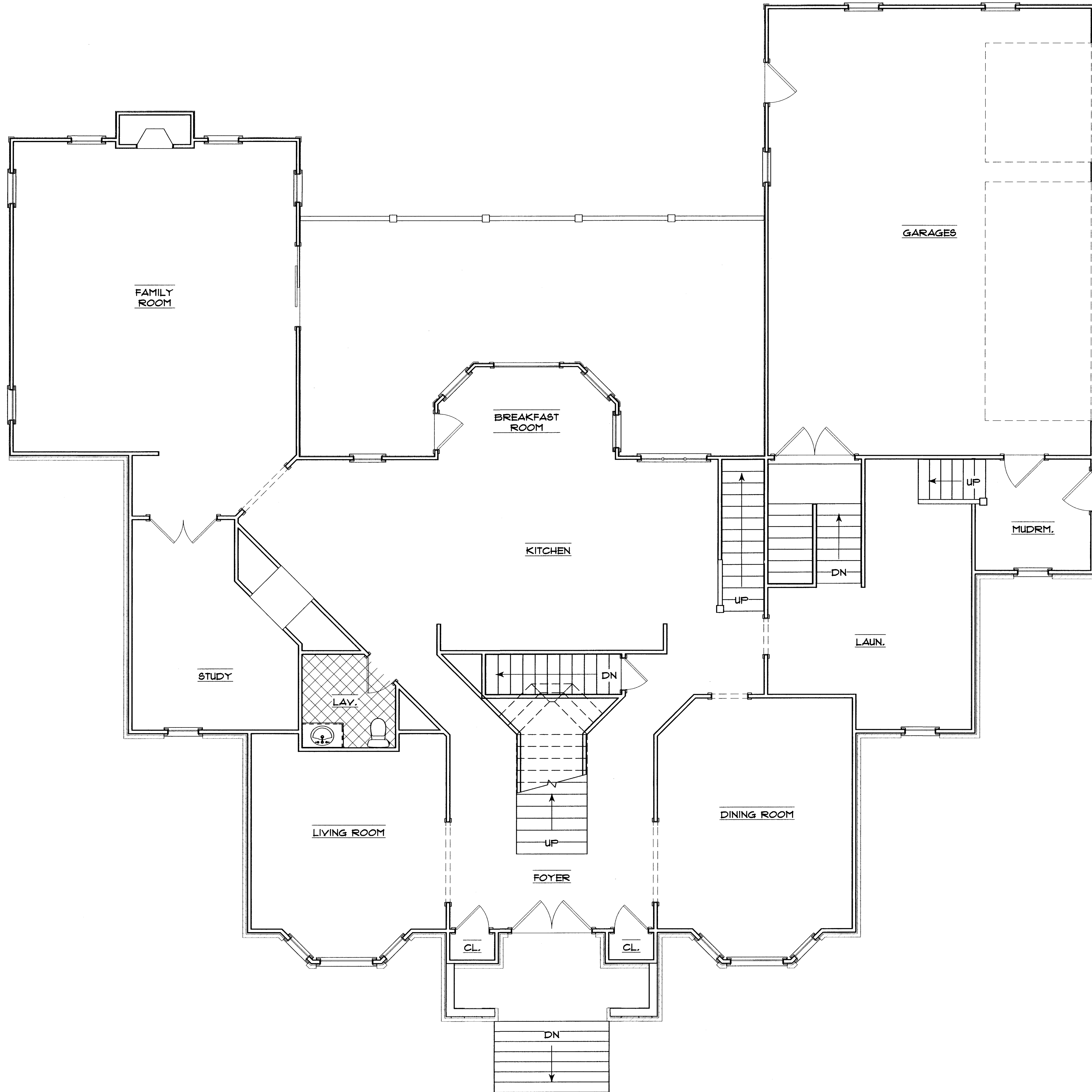
AS-BUILT FIRST FLOOR PLAN SCALE: 1/4" = 1'-0"
