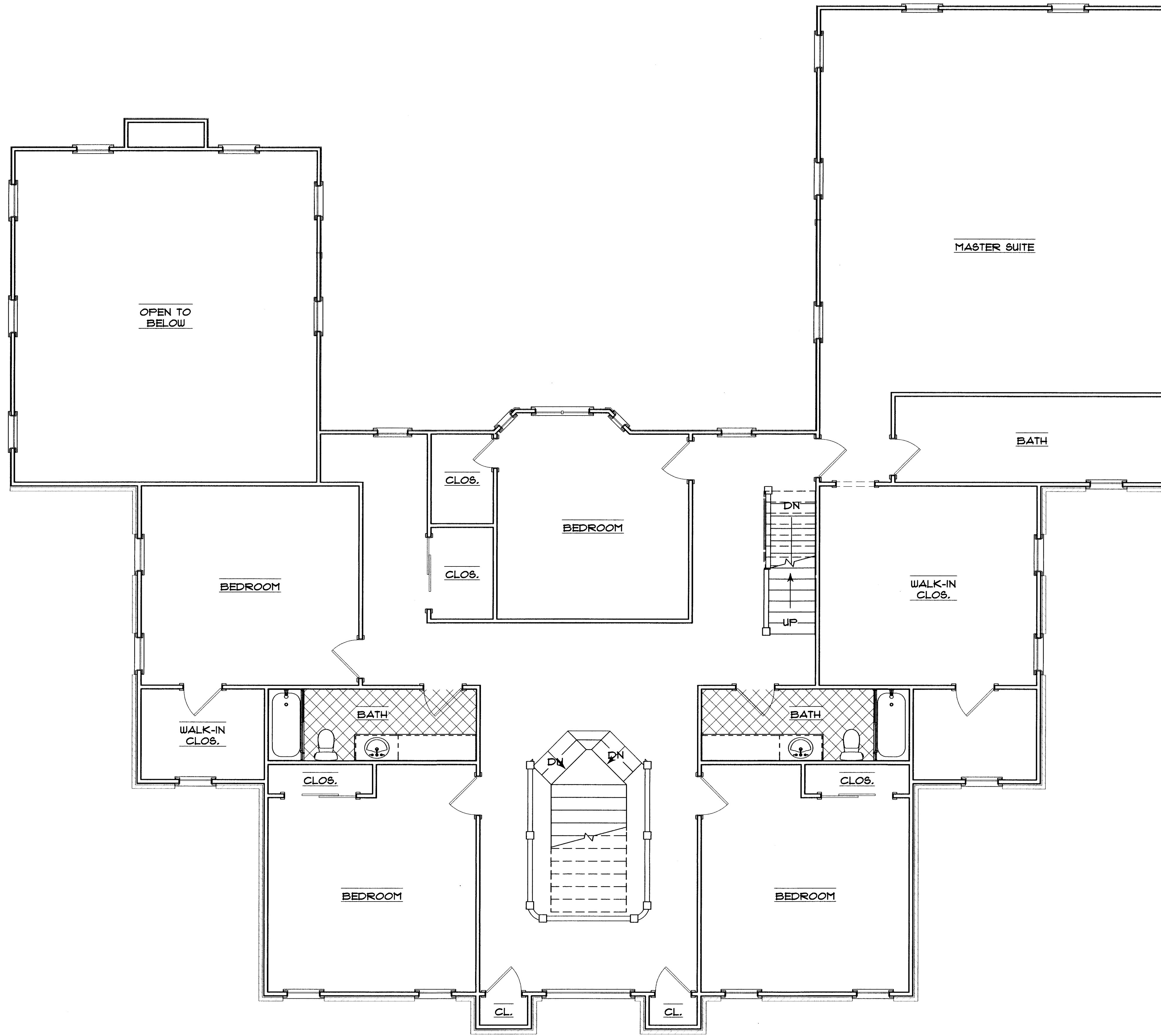
AS-BUILT SECOND FLOOR PLAN SCALE: 1/4" = 1'-0"
