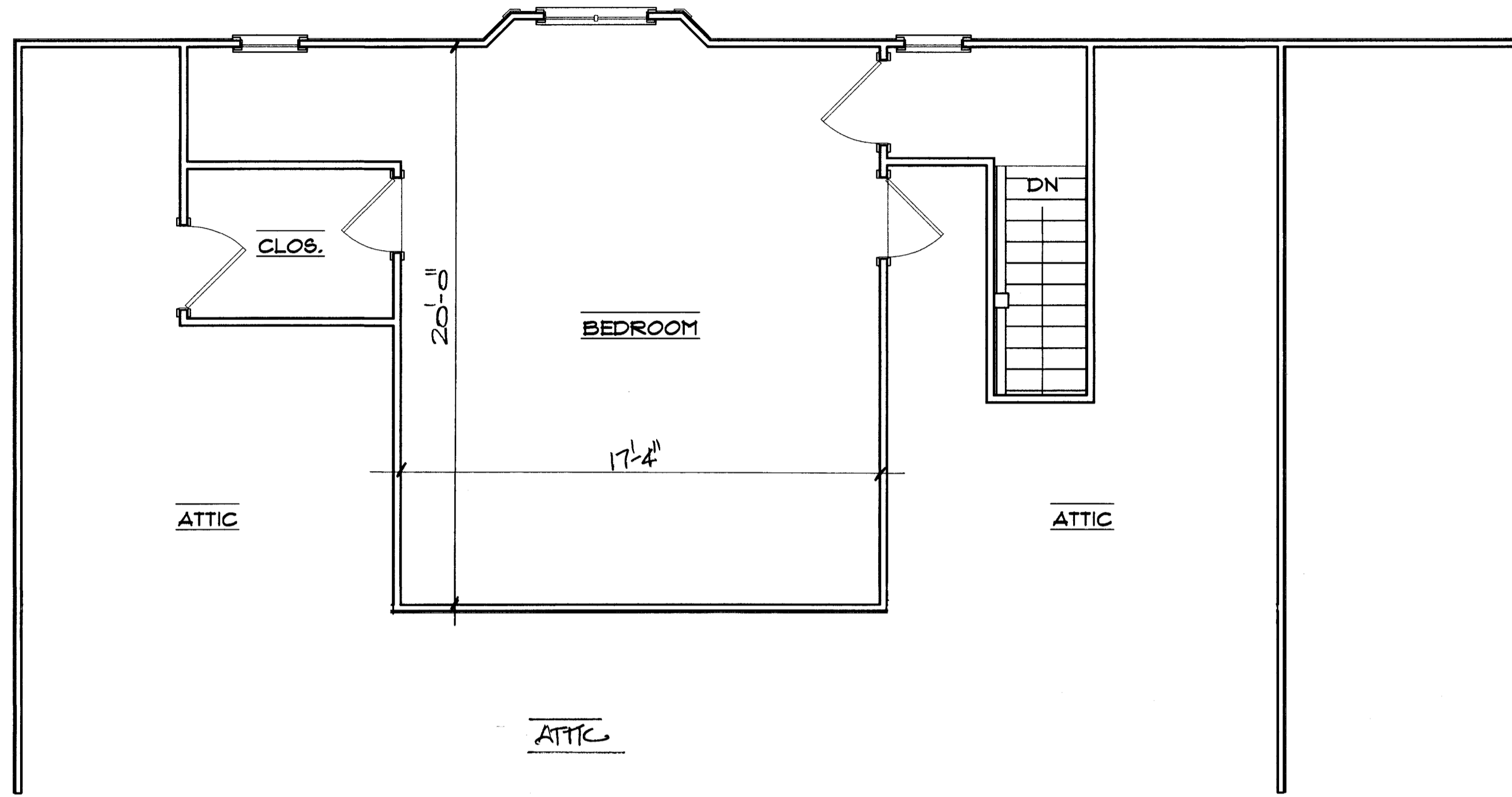
ATTIC FLOOR PLAN SCALE: 1/4" = 1'-0"
